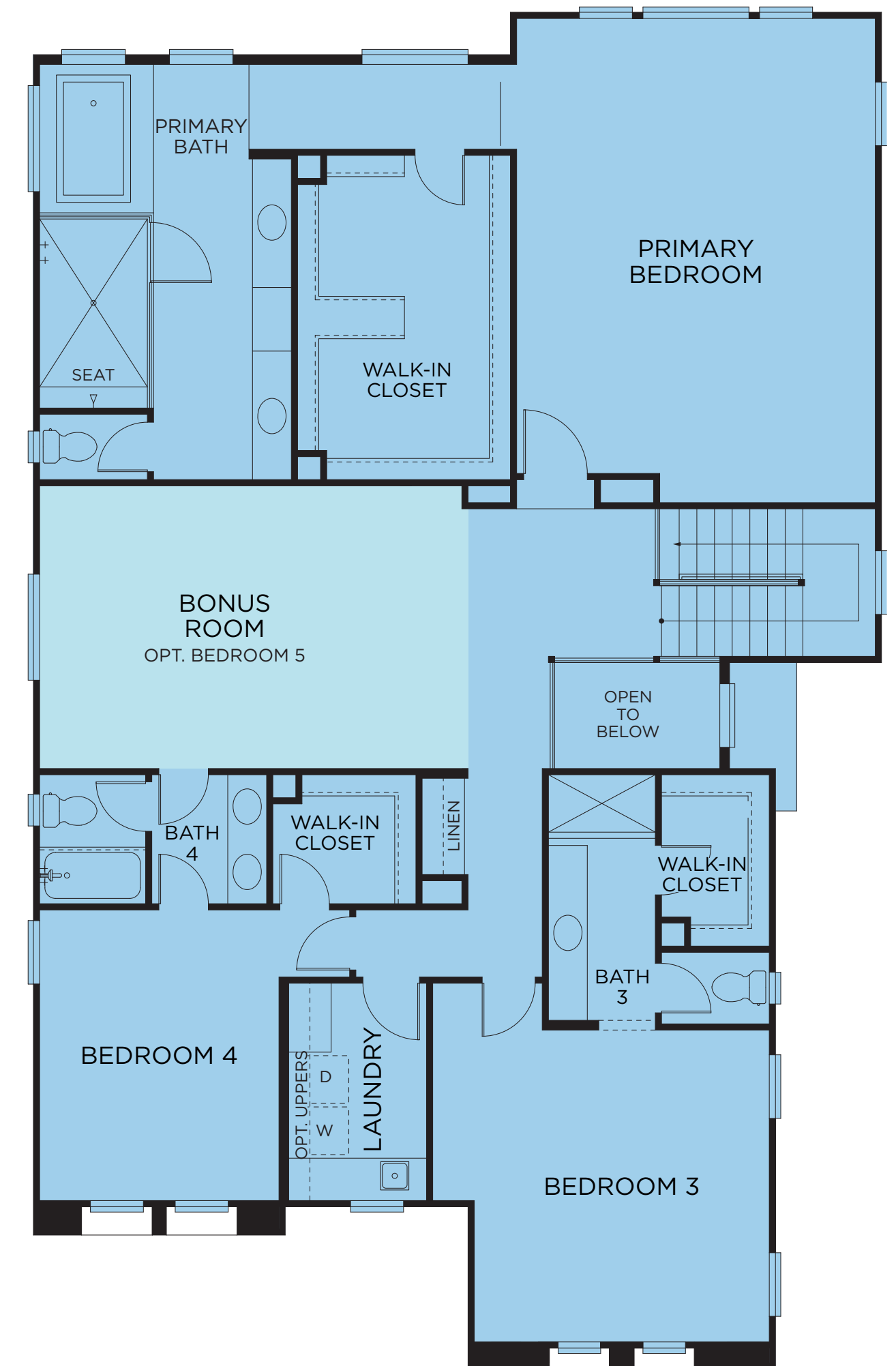
SECOND FLOOR
